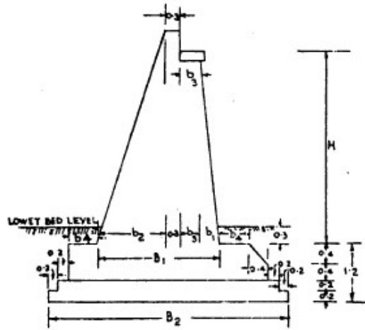
SECTION OF ABUTMENT
